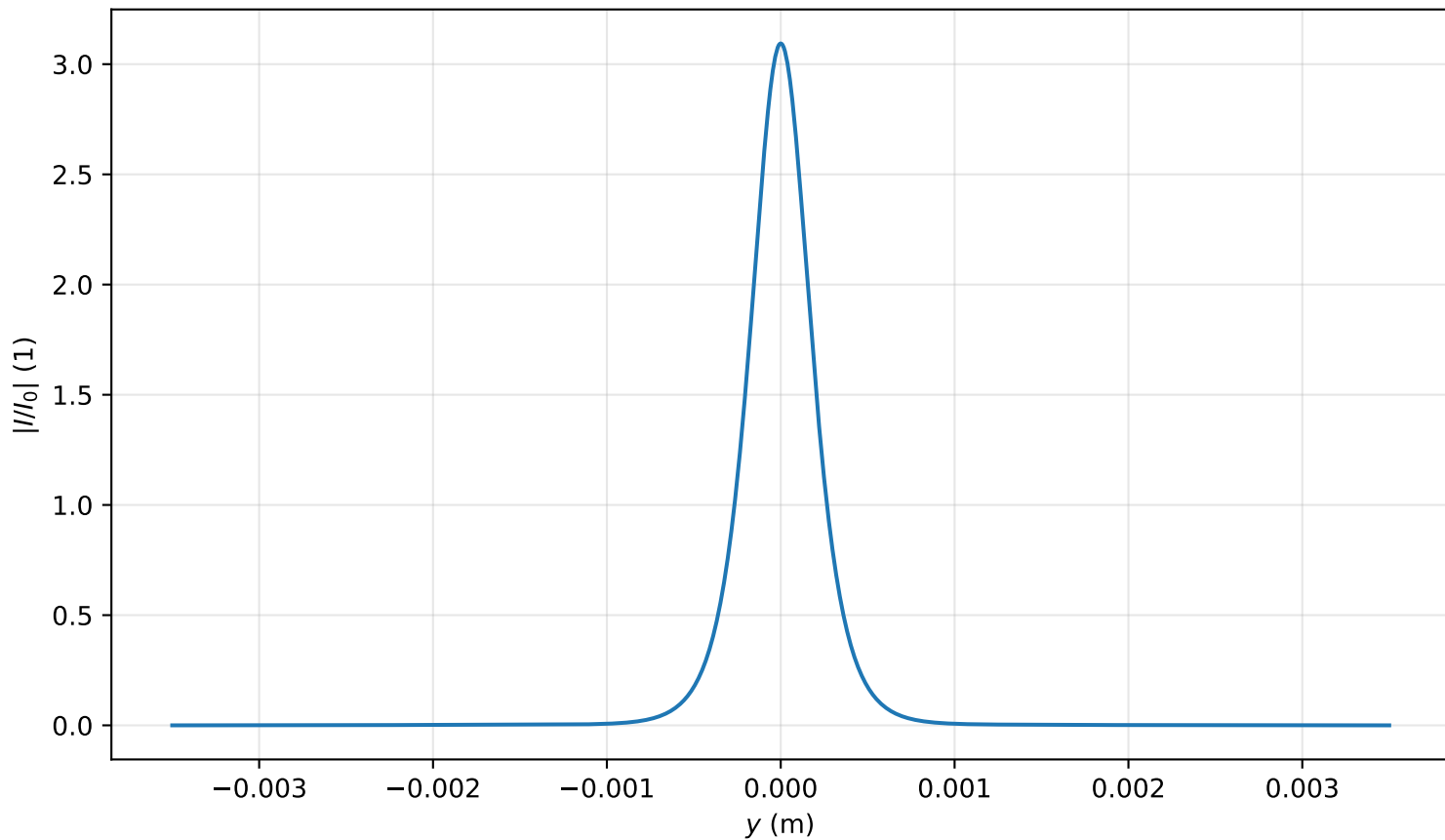
Intensity profile I(x=0, y, z=3.662)/I_0 , \text{Pin}=1.0\text{Pcr} , artificial time
